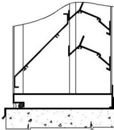
Channel W/sill
