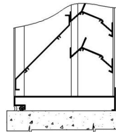
Channel Frame
